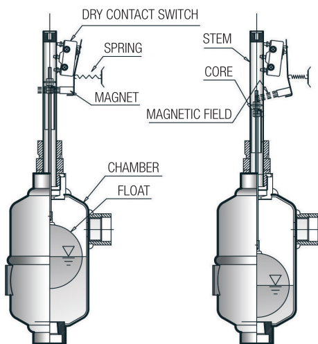
Fig.1. Switch Connected
